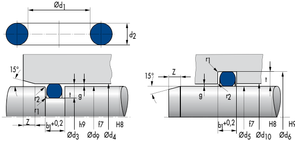
ISC O-Ring groove dimensions for fitting in hydraulics with axial/oscillating movements
