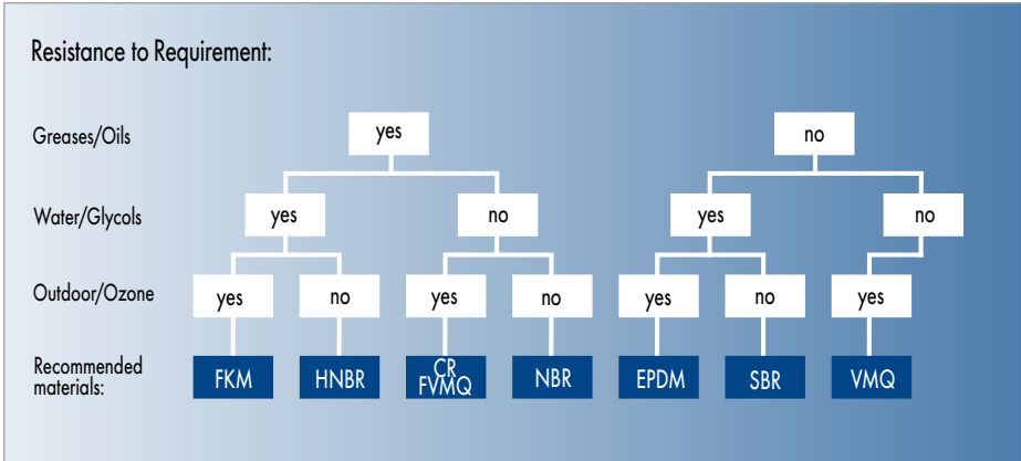
Material configuration
